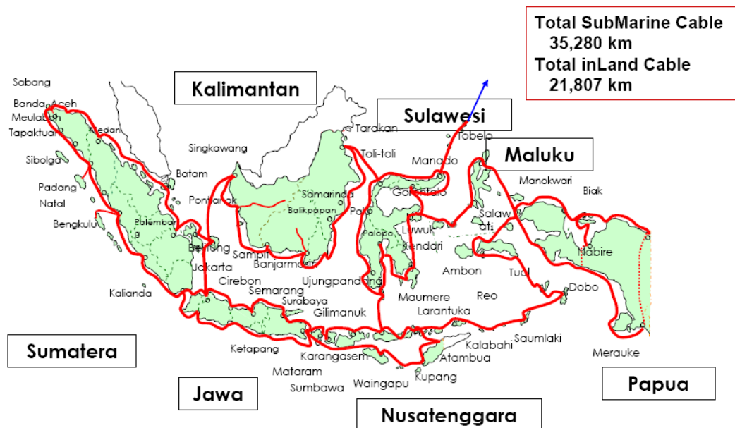
Figure 17 : Blueprint of (proposed) Palapa ring
